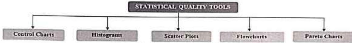
Fig.3 Statistical Quality Tools
