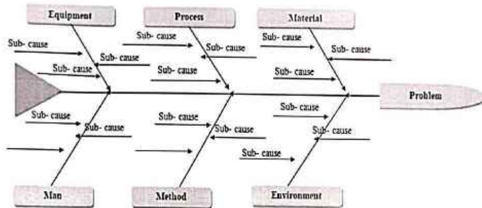
Fig. 7 Fishbone Diagram
