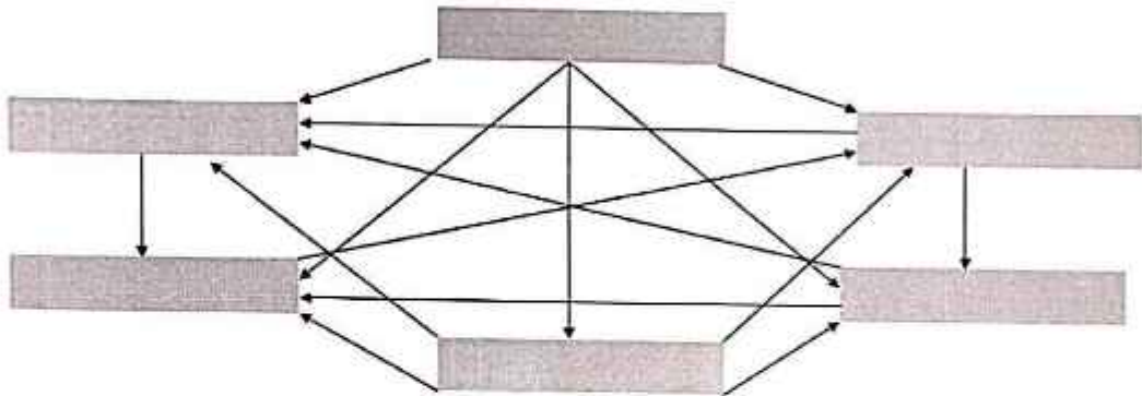
Fig. 10 Interrelationship Diagram
