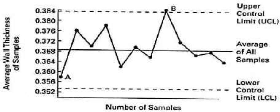
Fig. 4 Control Chart
