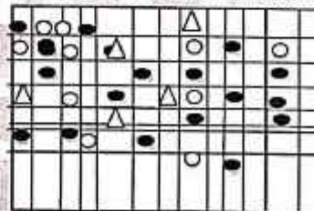
Fig. 11 Matrix Diagram
