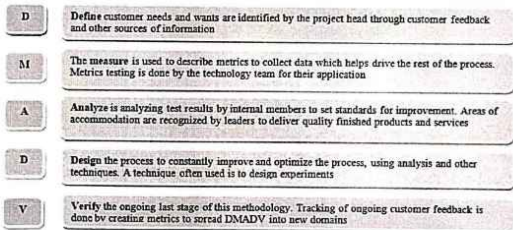
Fig.3 DMADV Methodology
