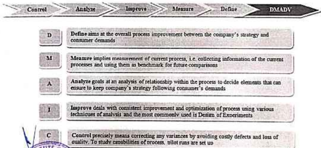
Fig.2 DMAIC Methodology
