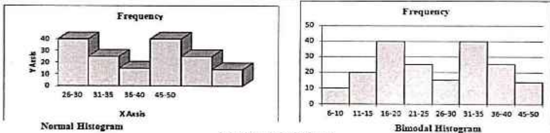
Fig. 5 Types of Histogram
