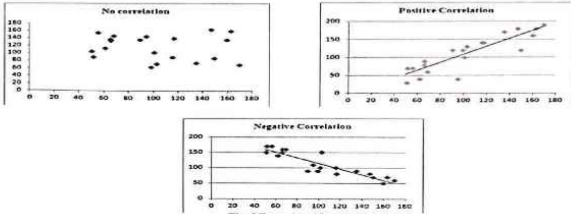
Fig. 5 Examples of Scatter Plot
